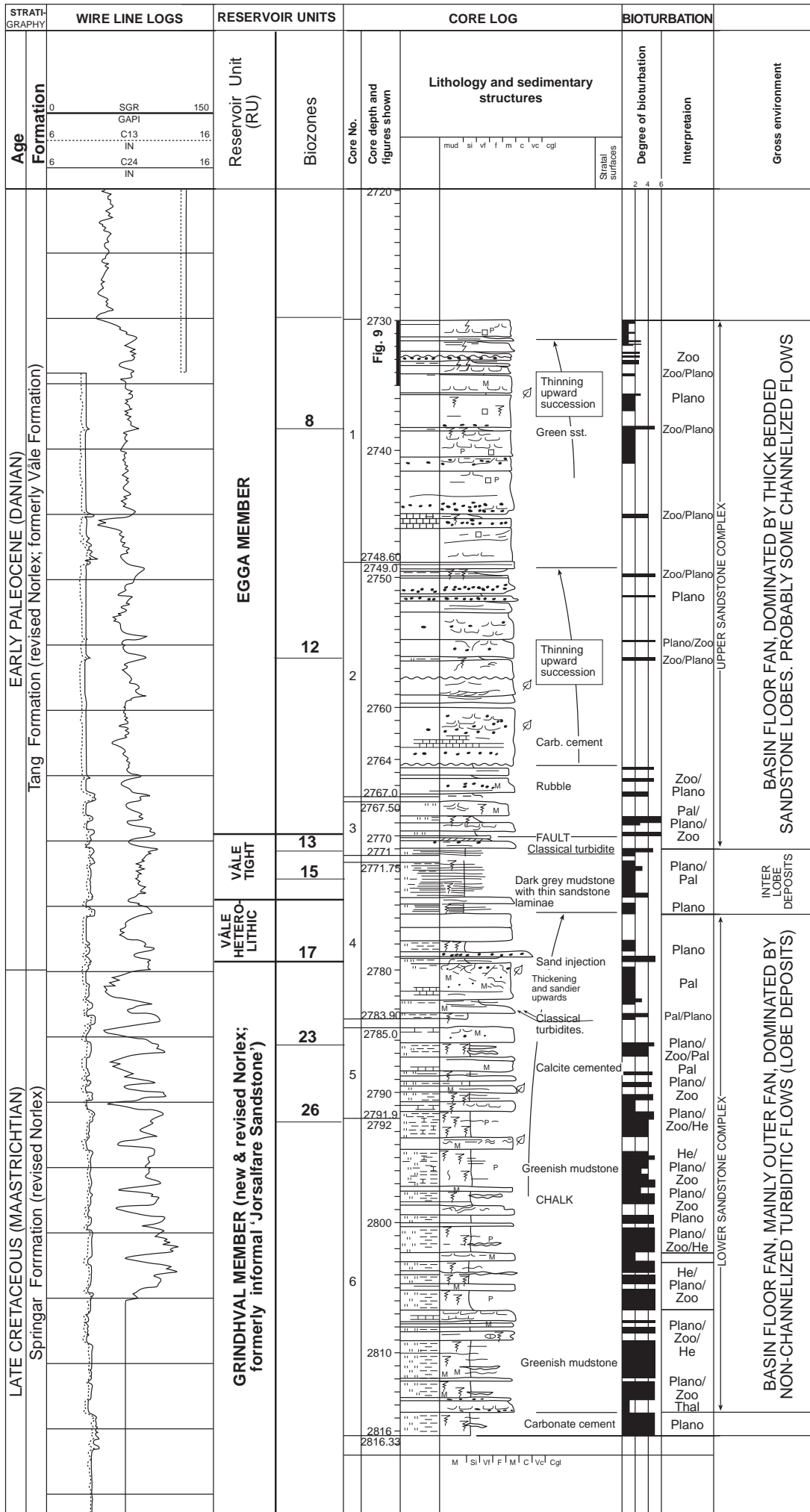
Core log of the Ormen Lange discovery well 6305/5-1 (Gjelberg et al., 2001, 2005; with modified Norlex lithostratigraphic terminology).
